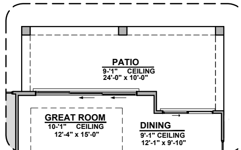
Stacking in Addition to Standard Door *EXTENDED PATIO HAS TO BE SELECTED
