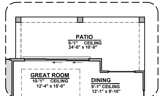
Stacking Door Ilo Standard Door *EXTENDED PATIO HAS TO BE SELECTED
